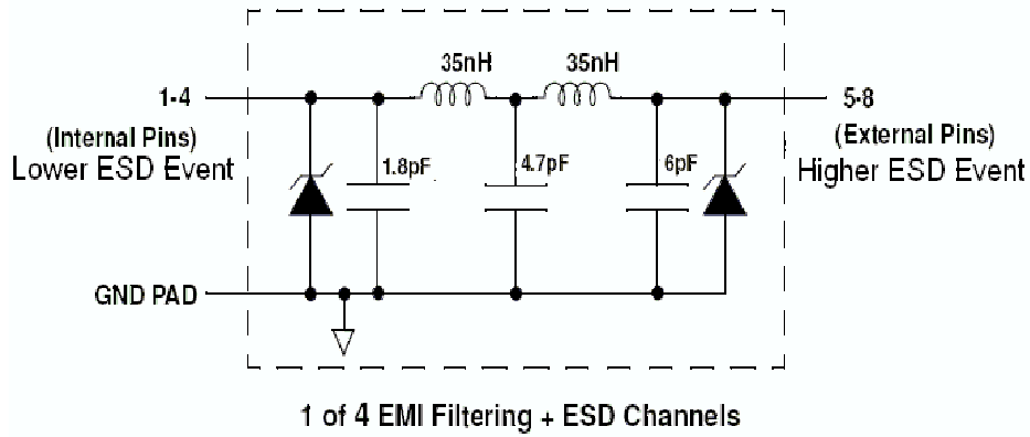
Figure 1. Electrical Schematic
